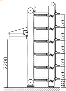
Standard Length 1600mm
