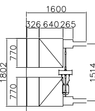
Standard Length 1600mm
